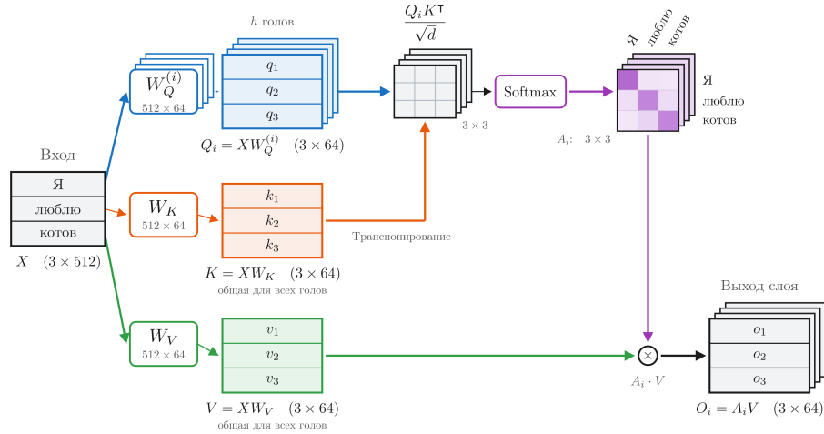
Рис. 68: Схема Multi-Query Attention.
